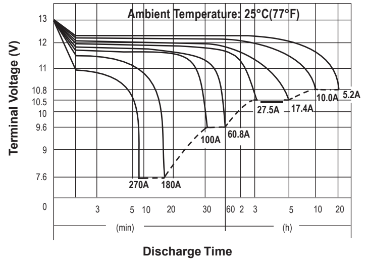
Discharge Characteristics
